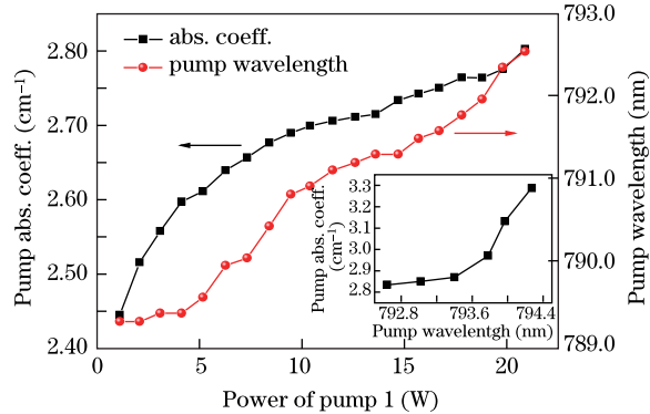
Fig. 2. Experimentally measured pump absorption coefficient under non-lasing conditions with the LD heat sink temperature maintained at 30 °C.
