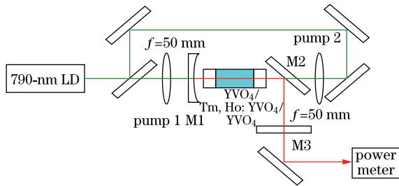
Fig. 1. Experimental setup of the composite Tm, Ho:YVO 4 laser.
