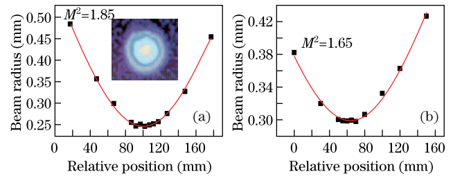
Fig. 6. Brightness determination of the Tm, Ho:YVO 4 laser, (a) composite Tm, Ho:YVO 4 crystal at 20-W output level, and (b) non-composite Tm, Ho:YVO 4 crystal at 14-W output level. Inset in (a), typical two-dimensional beam profiles taken using a Spiricon Pyrocam I pyroelectric camera.
