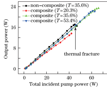
Fig. 3. Output power as a function of the total incident pump power for the composite and non-composite Tm, Ho:YVO 4 laser under different output mirror transmissions.
